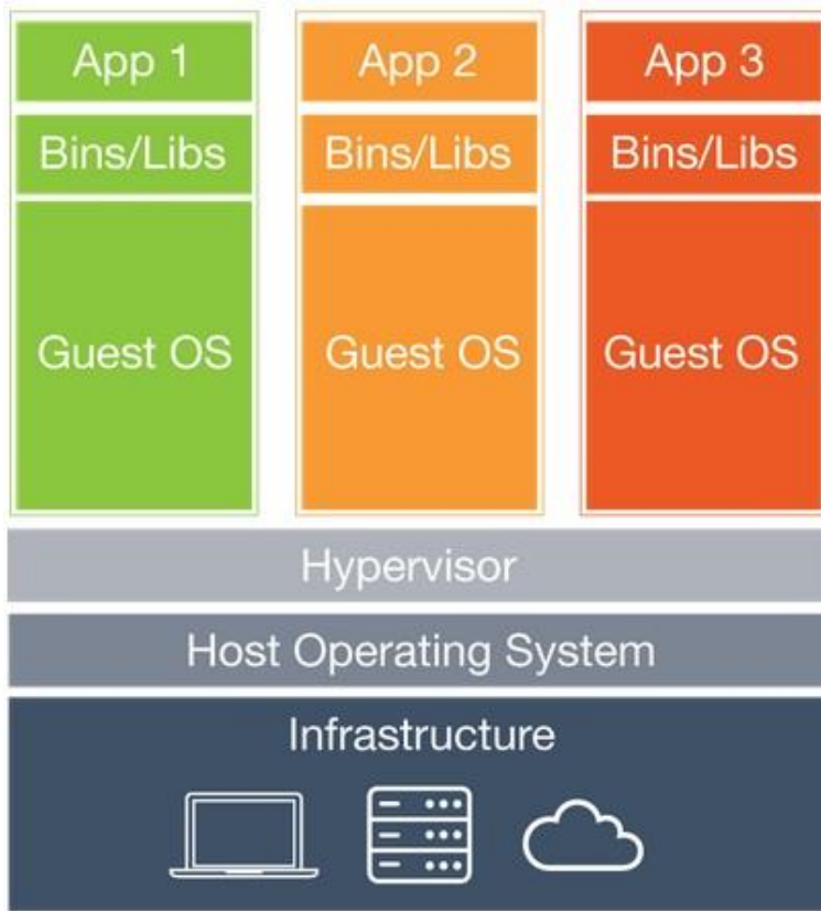
Virtual Machines
