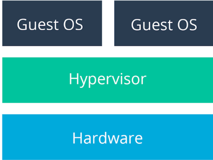
TYPE 1 HYPERVISOR
