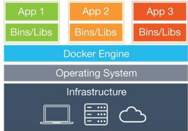
Containers
