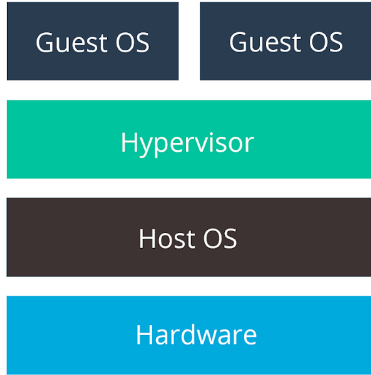
TYPE 2 HYPERVISOR
